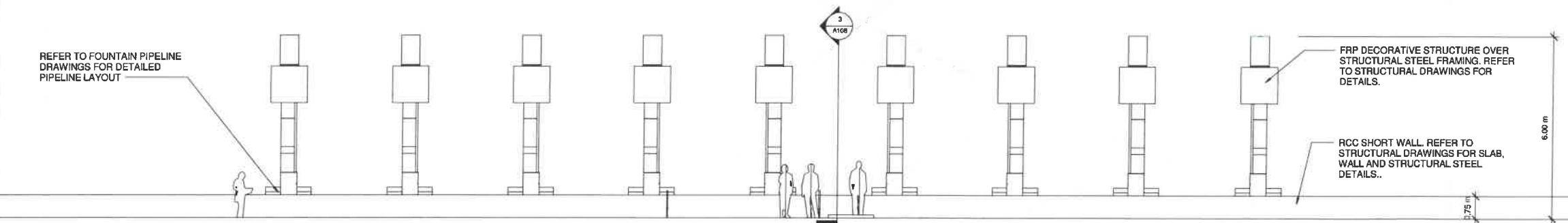
2 INDIAN STYLE FOUNTAIN - ELEVATION 1 : 75
