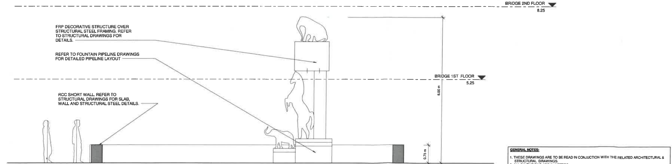
3 INDIAN FOUNTAIN - SECTION 1 : 40
