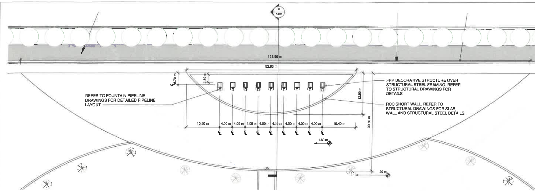
1 INDIAN STYLE FOUNTAIN - PLAN 1 : 300
